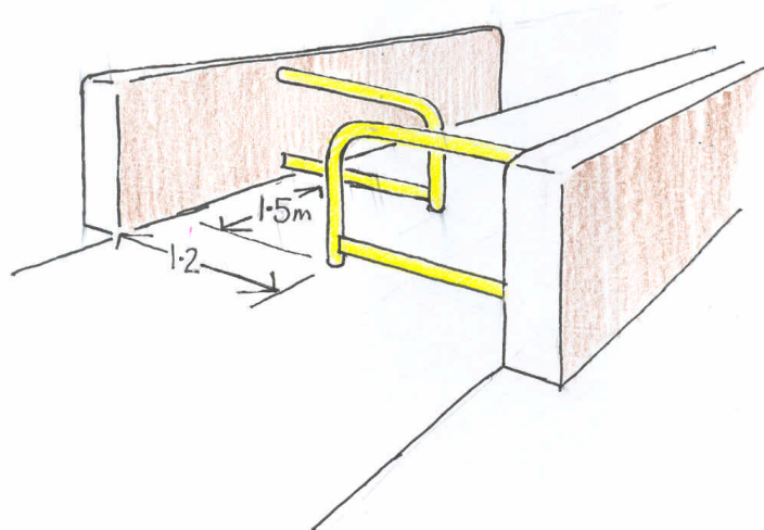
Minimum dimensions for chicane barrier
